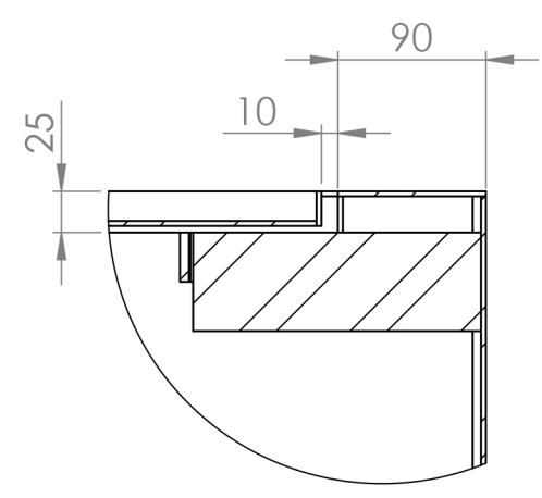
DETAIL K SCALE 1 : 5
