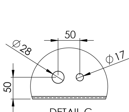
DETAIL C SCALE 1 : 5
