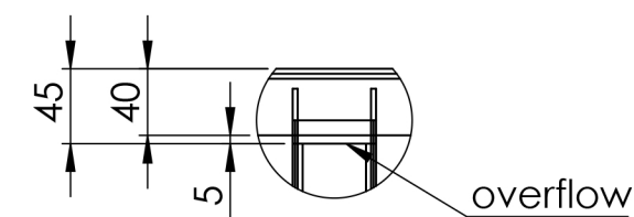
DETAIL A SCALE 1 : 5
