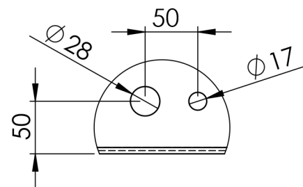
DETAIL C SCALE 1 : 5
